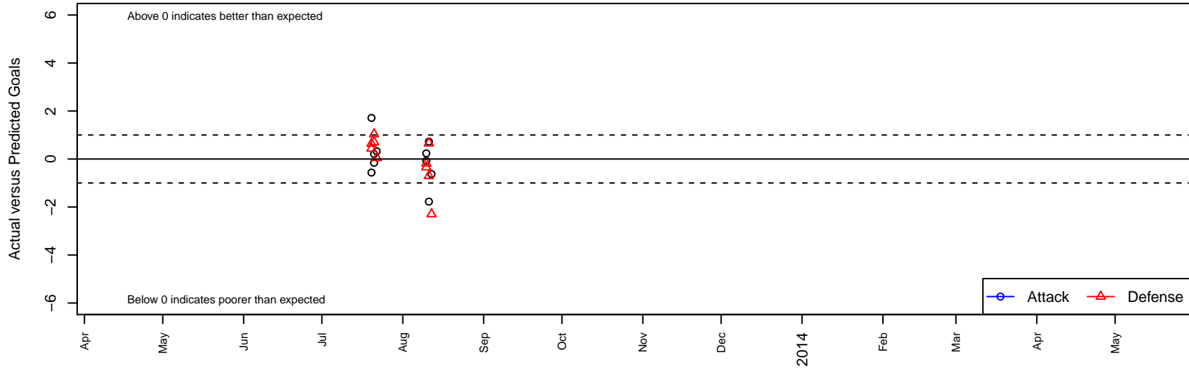
Arizona Hammers 99 Elite B98 Dots are actual minus expected GF (blue circles) and GA (red triangles). Blue line is smoothed change in attack strength. Red is smoothed change in defense strength.
